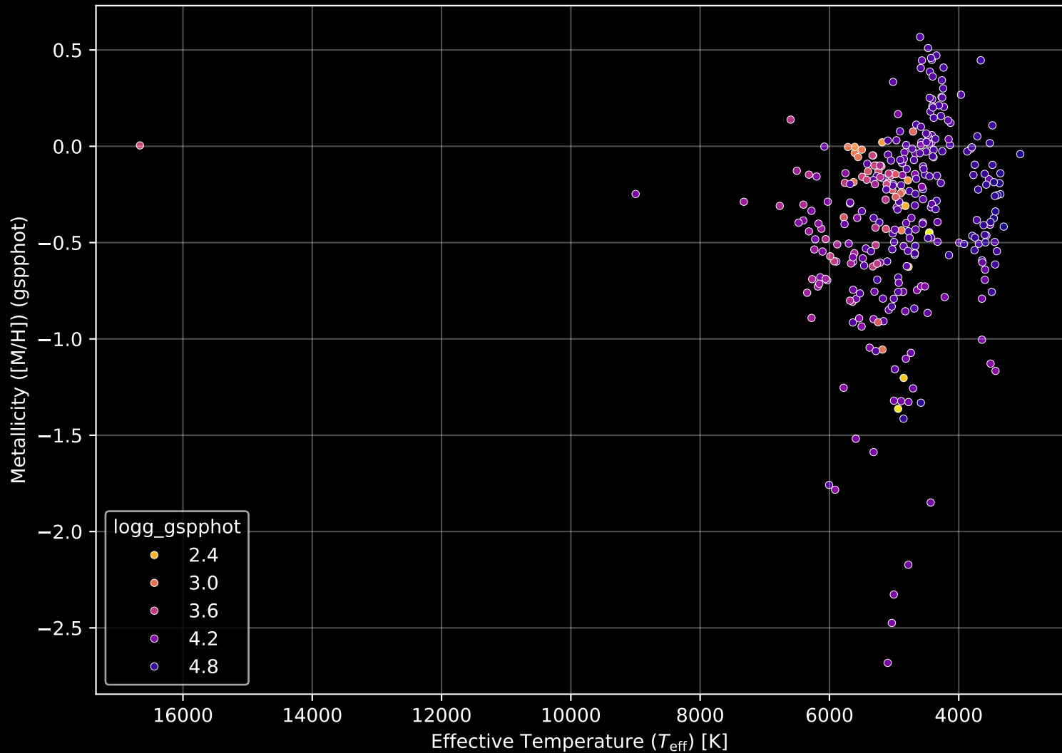
APOGEE DR17 Field: [ORPHAN-2] Stellar Population Parameters (n= 317)
