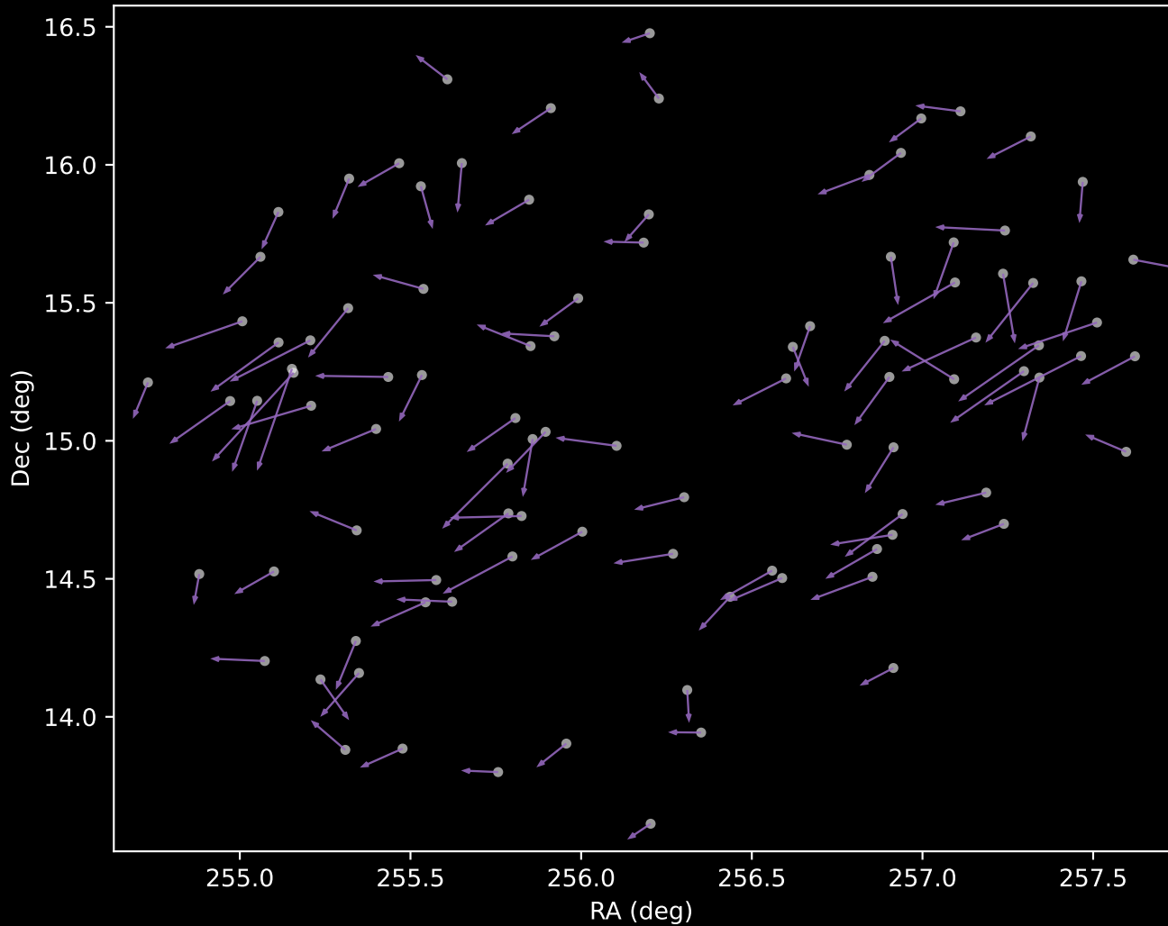
APOGEE DR17 Cluster 8 Proper Motion Vectors (n=98)
