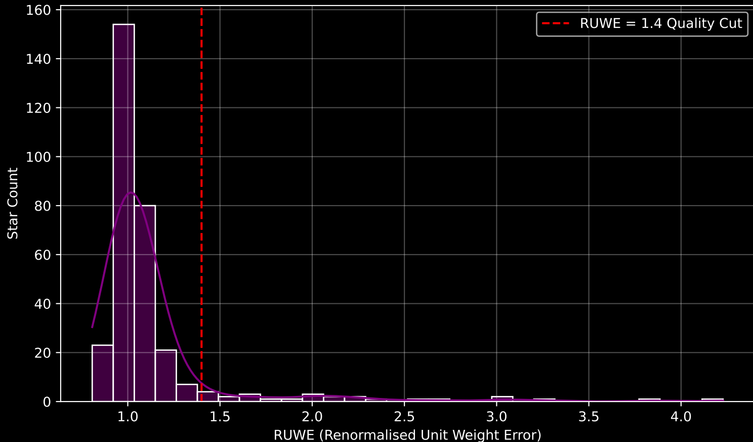
GAPOGEE DR17 Field [ORPHAN-2] RUWE Distribution (n= 311)
