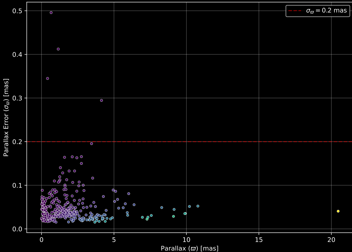
APOGEE DR17 Field: [ORPHAN-2] Parallax Quality (n= 317)
