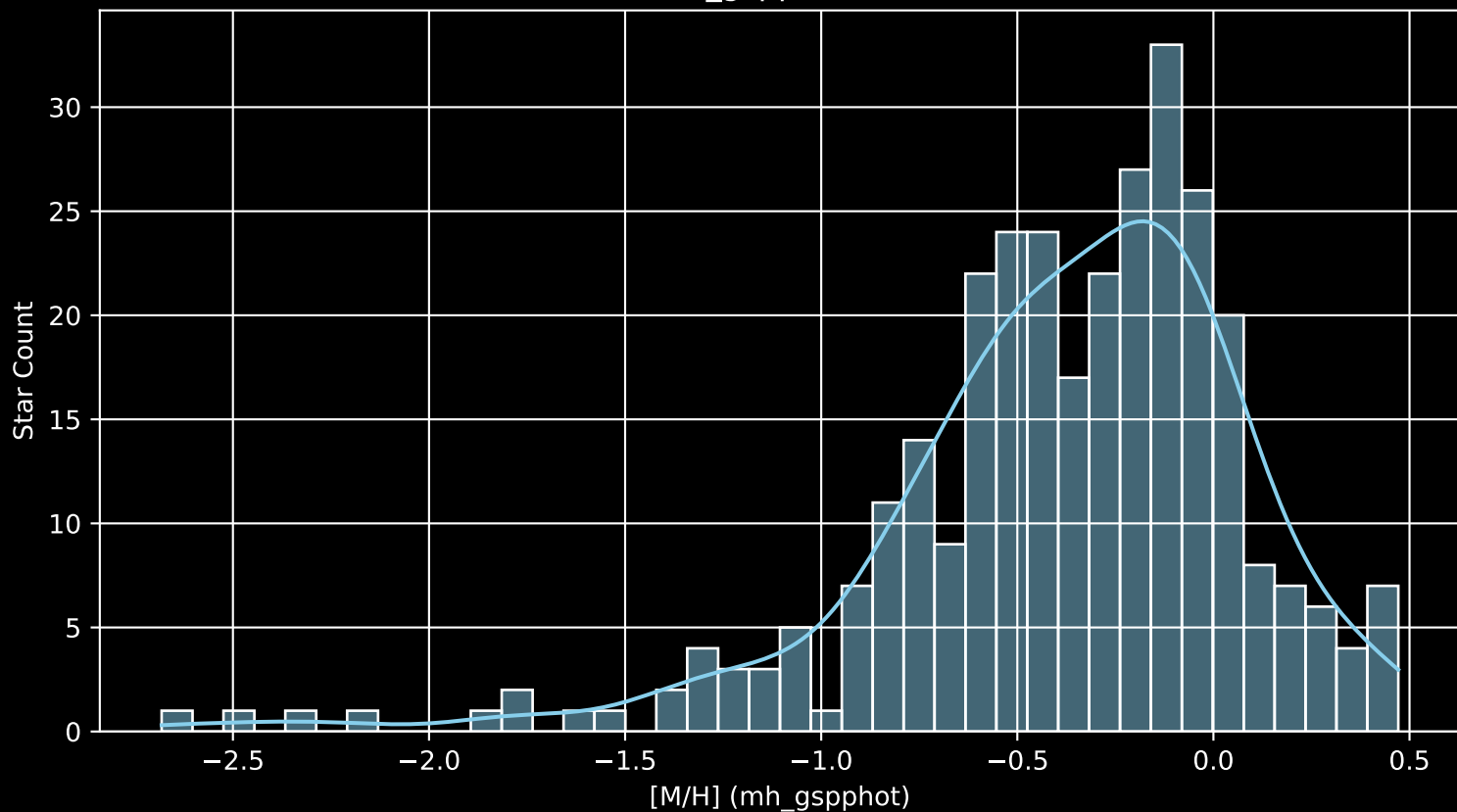
APOGEE DR17 Field: [ORPHAN-2 [M/H] (mh_gspphot) (n= 315)
