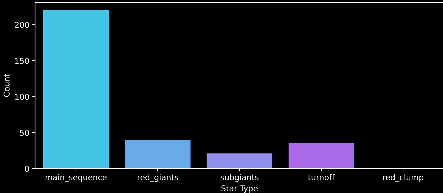
APOGEE DR17 Field: [ORPHAN-2] Count plot of Star Type
